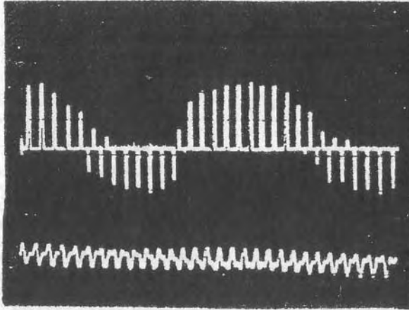
Figure 3. Two 1 second traces of ambient magnetic field impulses gathered in California with a coil detection system and displayed in the time domain on a storage oscilloscope. Top trace railed; bottom trace normalized headroom. Note the variable polarity serpentine like characteristics similar to Figure 2.
