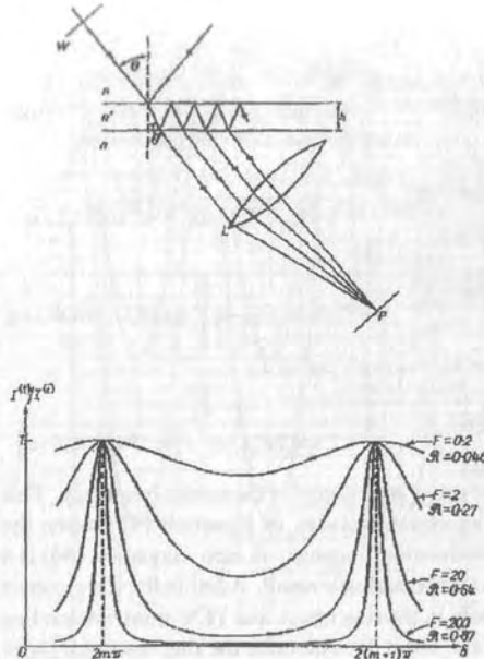
Figure 10. (a) Formation of multiple beam fringes in a parallel plate of index of refraction n' , focused to give the transmitted intensity (power density) I' . (b) The Airy function - a plot of the ratio of the transmitted and incident intensities as a function of the propagation path-produced phase difference \delta = 4\pi n' \cos \theta / \lambda_0 . [Ref. Born and Wolf, pp. 326-7. Script R is the power reflection coefficient r' and F = 4R / (1-R)^2 .]
